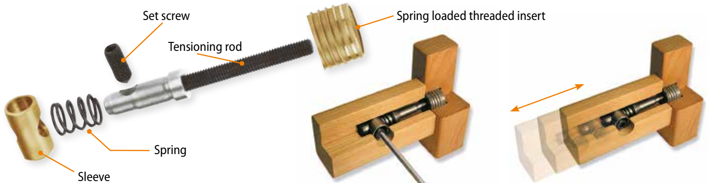
Example of table leg to table top connection
