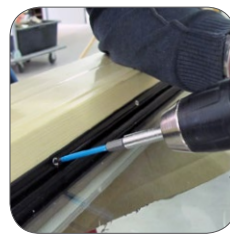
2) Visser FIXclip-Barre
