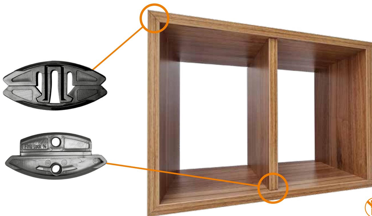
Drive in the connector, flush with the board using the insert tool.
