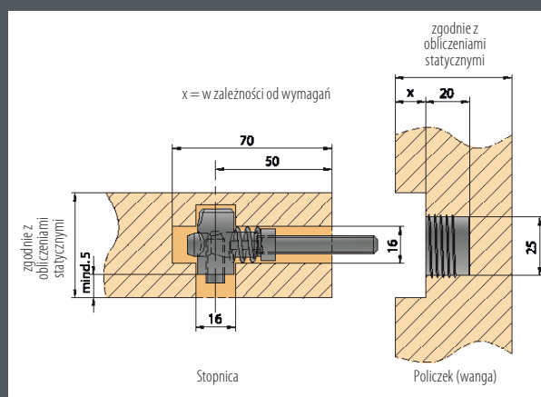
easy-con® M8-16-50
