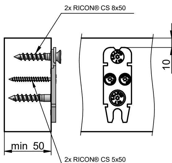
Locking clip assembly
