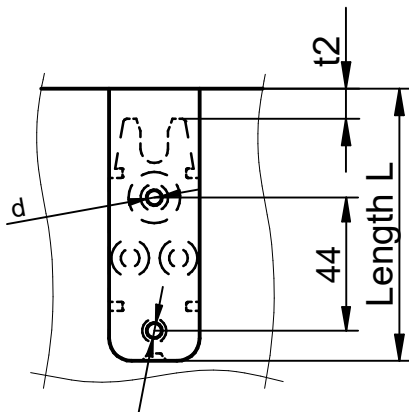
drilling pattern for main beam
