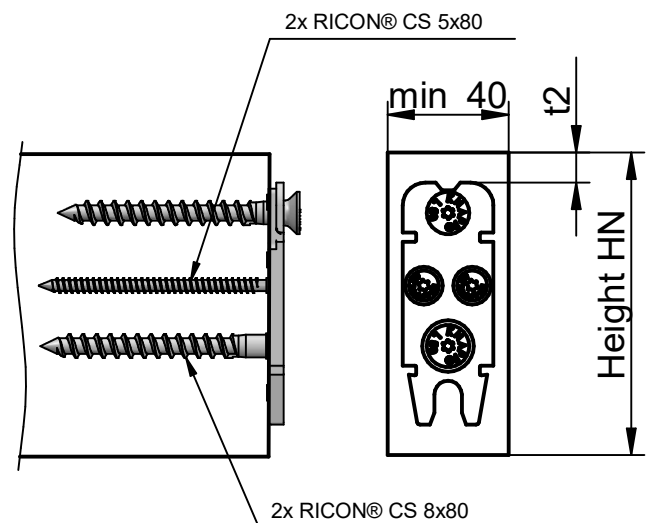
Locking clip assembly
