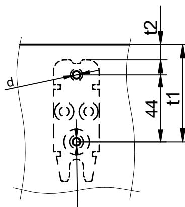
drilling pattern for secondary beam
