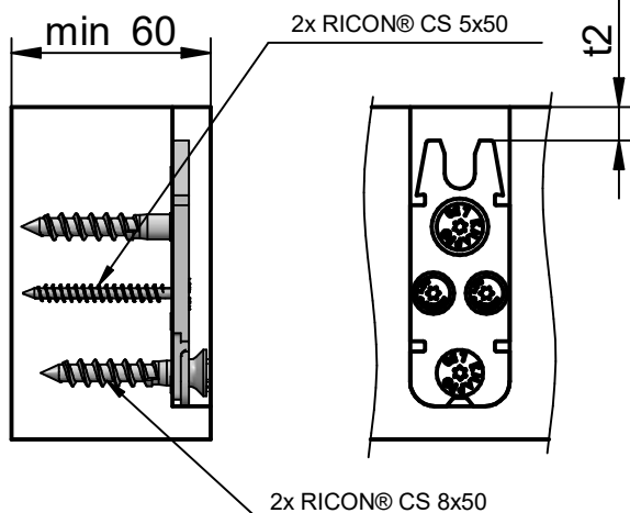
screw depth adjustable
