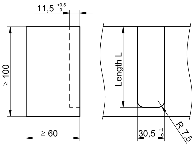
Milling pattern main beam
