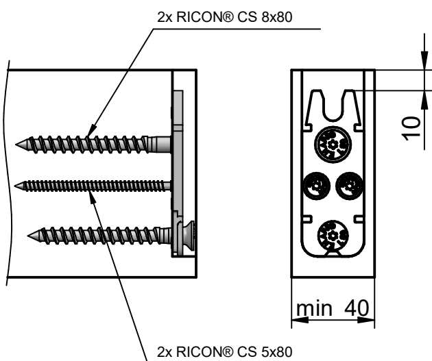
screw depth adjustable
