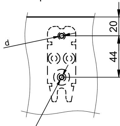
drilling pattern for post
