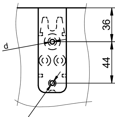
drilling pattern for beam
