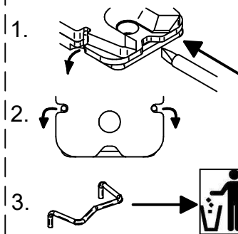
Locking clip removal
