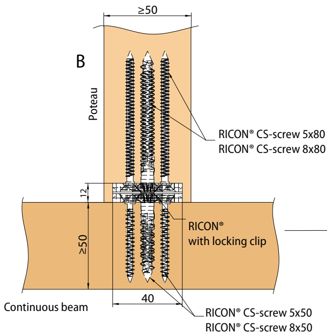
RICON® single connection (EA)
