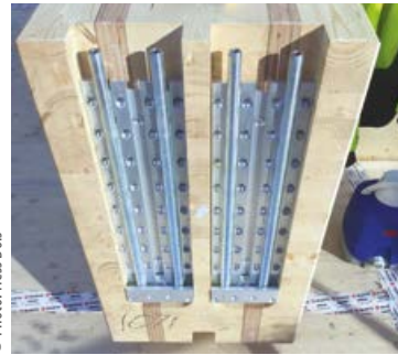
Three-sided concealed assembly by milling into the secondary beam. MEGANT® is fixed to the main beam with no need for milling.
