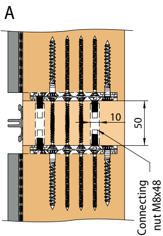
RICON® double connection (DA)
