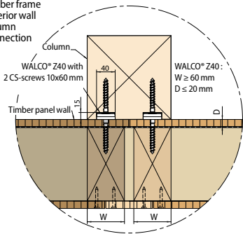
Detail D : Timber frame interior wall connection
