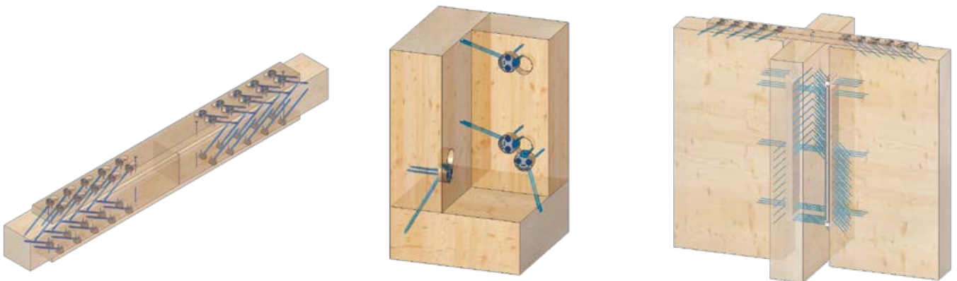
T-JOINT D35 W30 fastened hardwood tension ties for BSH tension joints.
