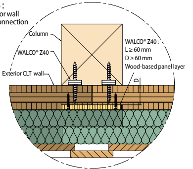
Detail D : CLT interior wall connection
